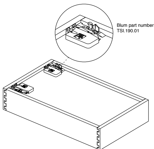
Blum TANDEM Clips Installed
