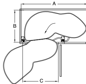
Swings Left
